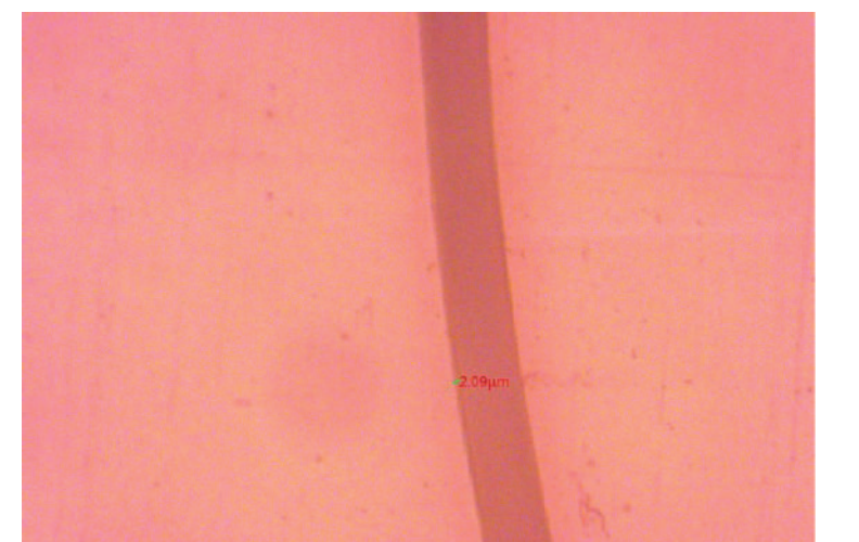
PI Film Cutting( 2.09\mu\text{m} )
